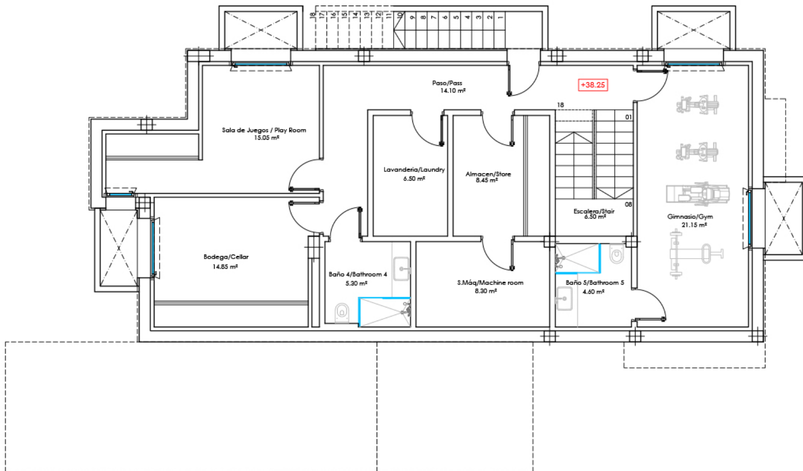
BASEMENT FLOOR
